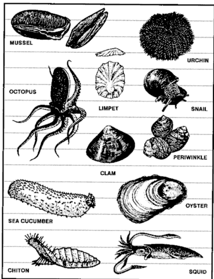
Figure 8-1. Edible mollusks.
