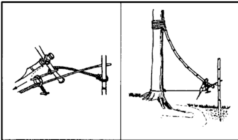
Figure 8-15. Pig spear shaft.
