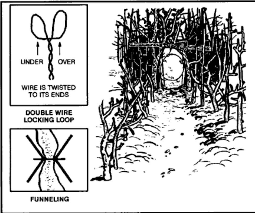
Figure 8-6. Drag noose.
