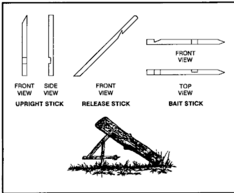
Figure 8-12. Figure 4 deadfall.
