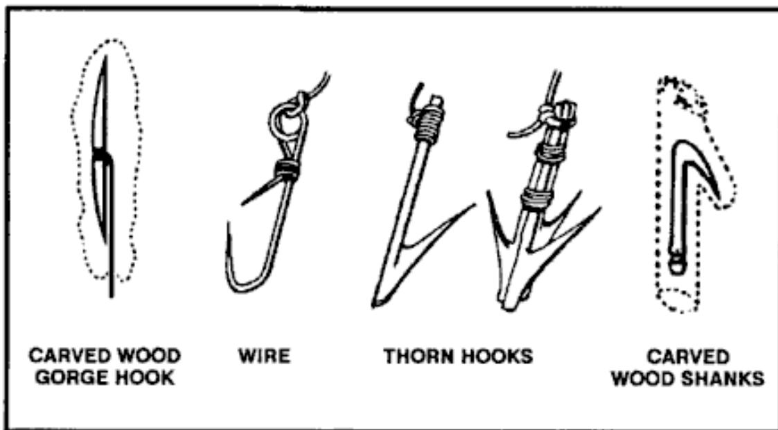
Figure 8-17. Improved fishhooks.
